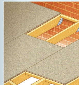
SE panels are laid with long edges in-line with the joists
