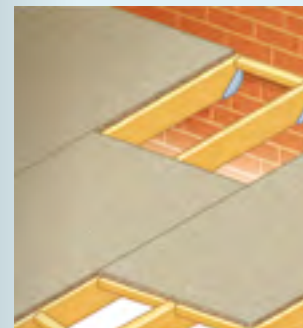
SE panels are laid with long edges in-line with the joists
